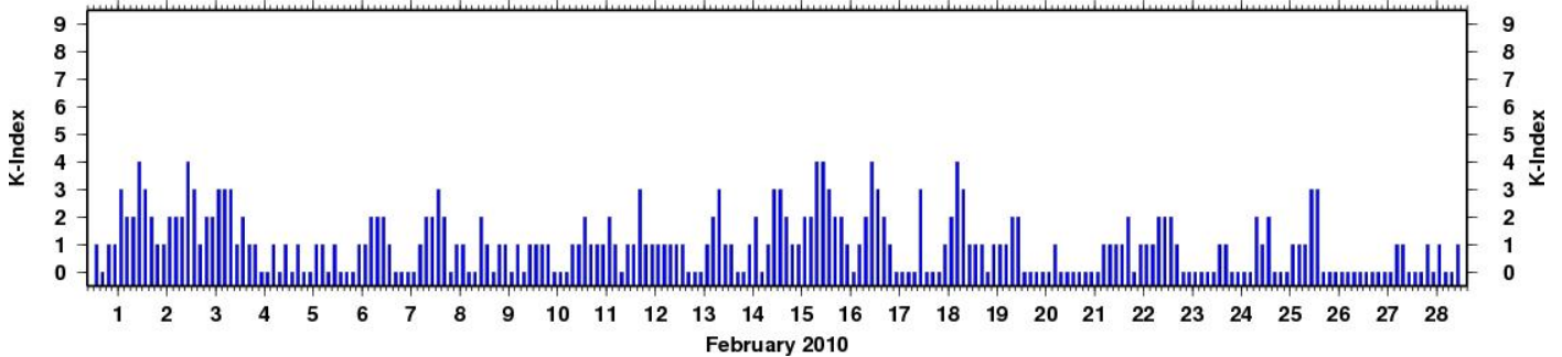
Hartland Observatory 3-hourly K-Indices
