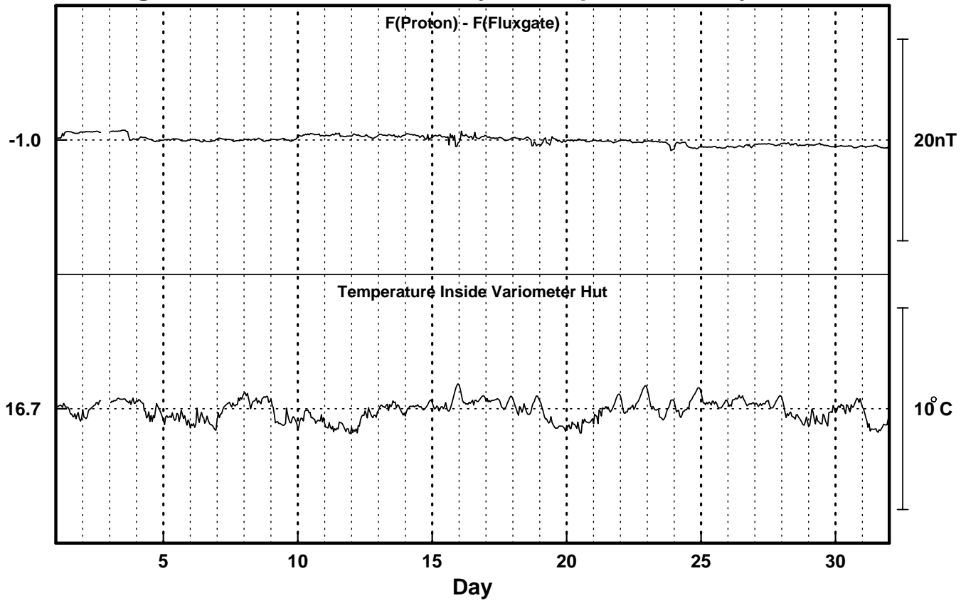
Figure 2 : Sable Island Monthly F Comparison July 2000
