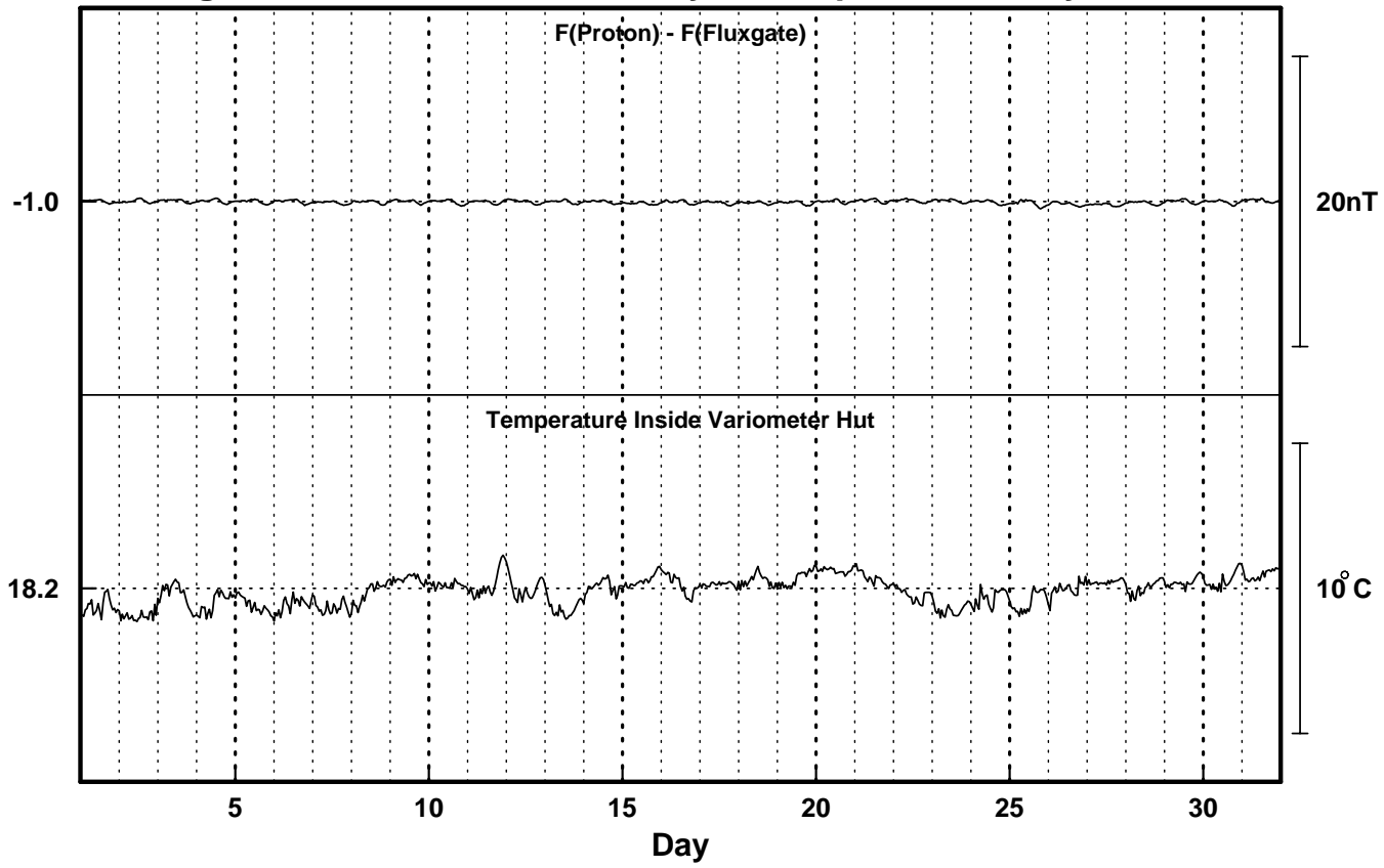
Figure 2 : Sable Island Monthly F Comparison July 2001
