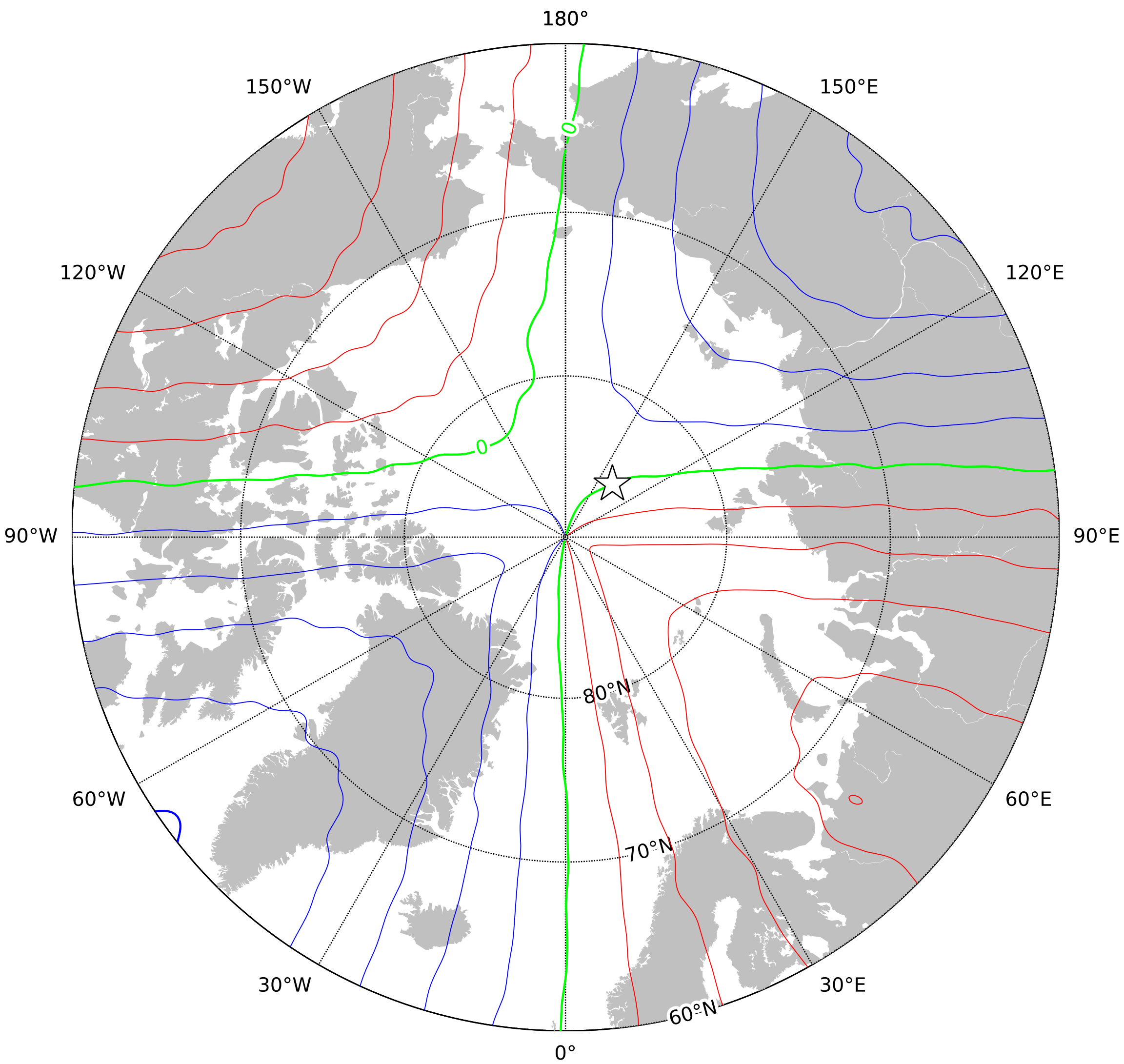
East component (Y) in the region of the north pole at 2025.0 from the World Magnetic Model - High Resolution (WMMHR) 2025. Red - positive (east), blue - negative (west), green - zero. Contour interval is 1000nT, white star is the location of a magnetic pole and the projection is Polar Stereographic. This is an example of an isodynamic chart.
