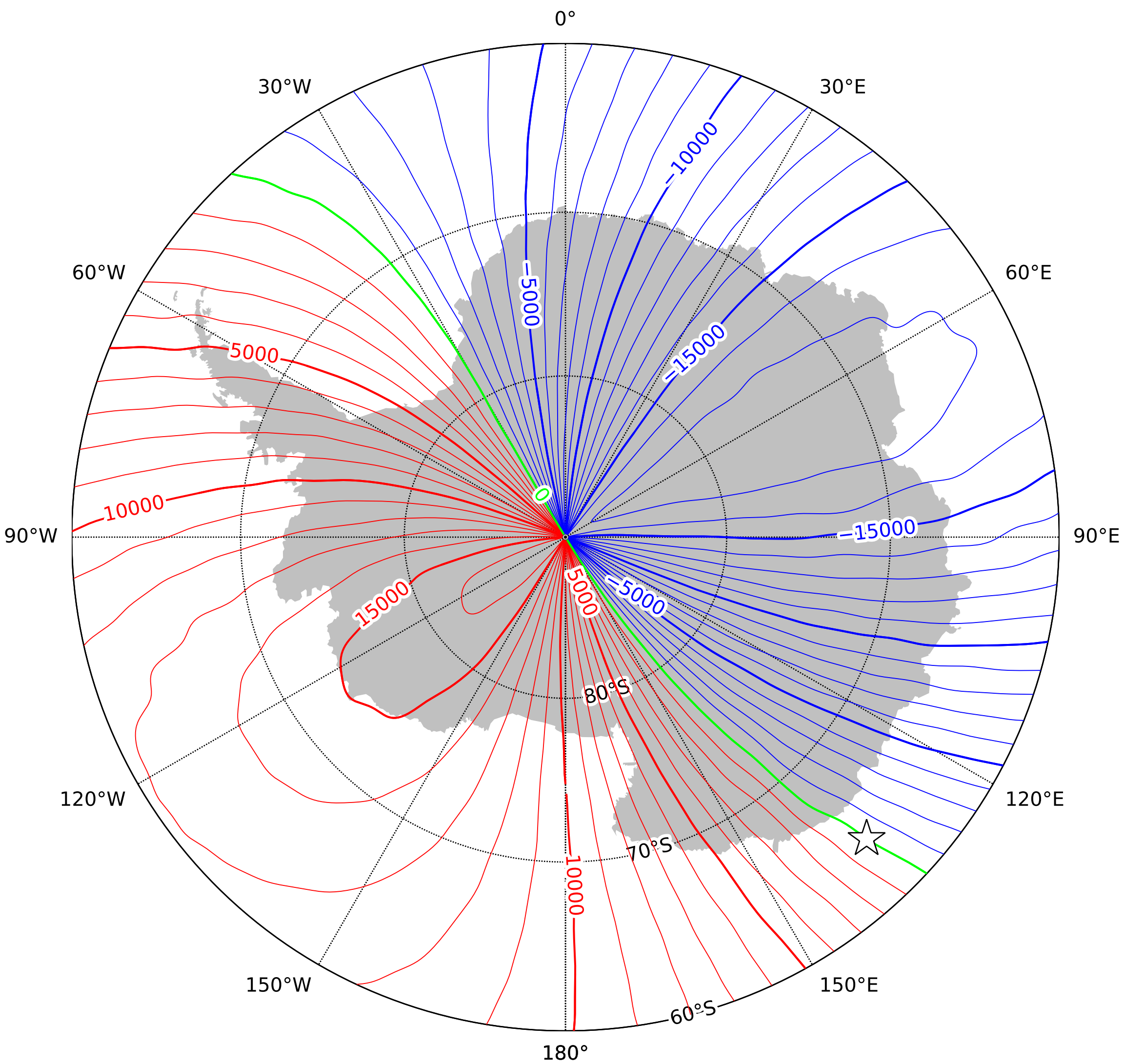
East component (Y) in the region of the south pole at 2025.0 from the World Magnetic Model - High Resolution (WMMHR) 2025. Red - positive (east), blue - negative (west), green - zero. Contour interval is 1000nT, white star is the location of a magnetic pole and the projection is Polar Stereographic. This is an example of an isodynamic chart.
