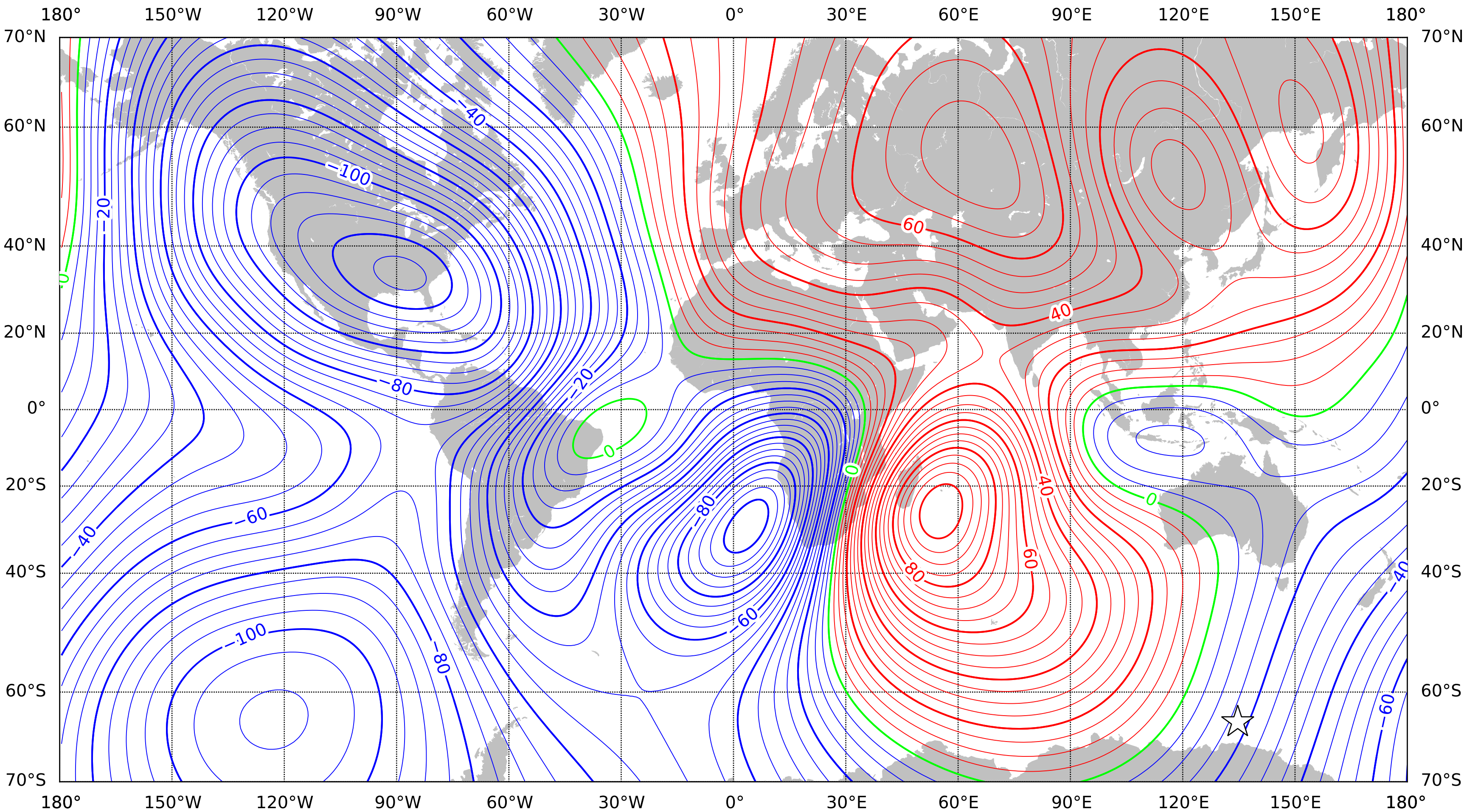
Annual rate of change of total intensity at 2027.5 from the World Magnetic Model - High Resolution (WMMHR) 2025 (core component only). Red - positive change, blue - negative change, green - zero change. Contour interval is 5nT/year, white star is the location of a magnetic pole and the projection is Mercator. This is an example of an isoporic chart.
