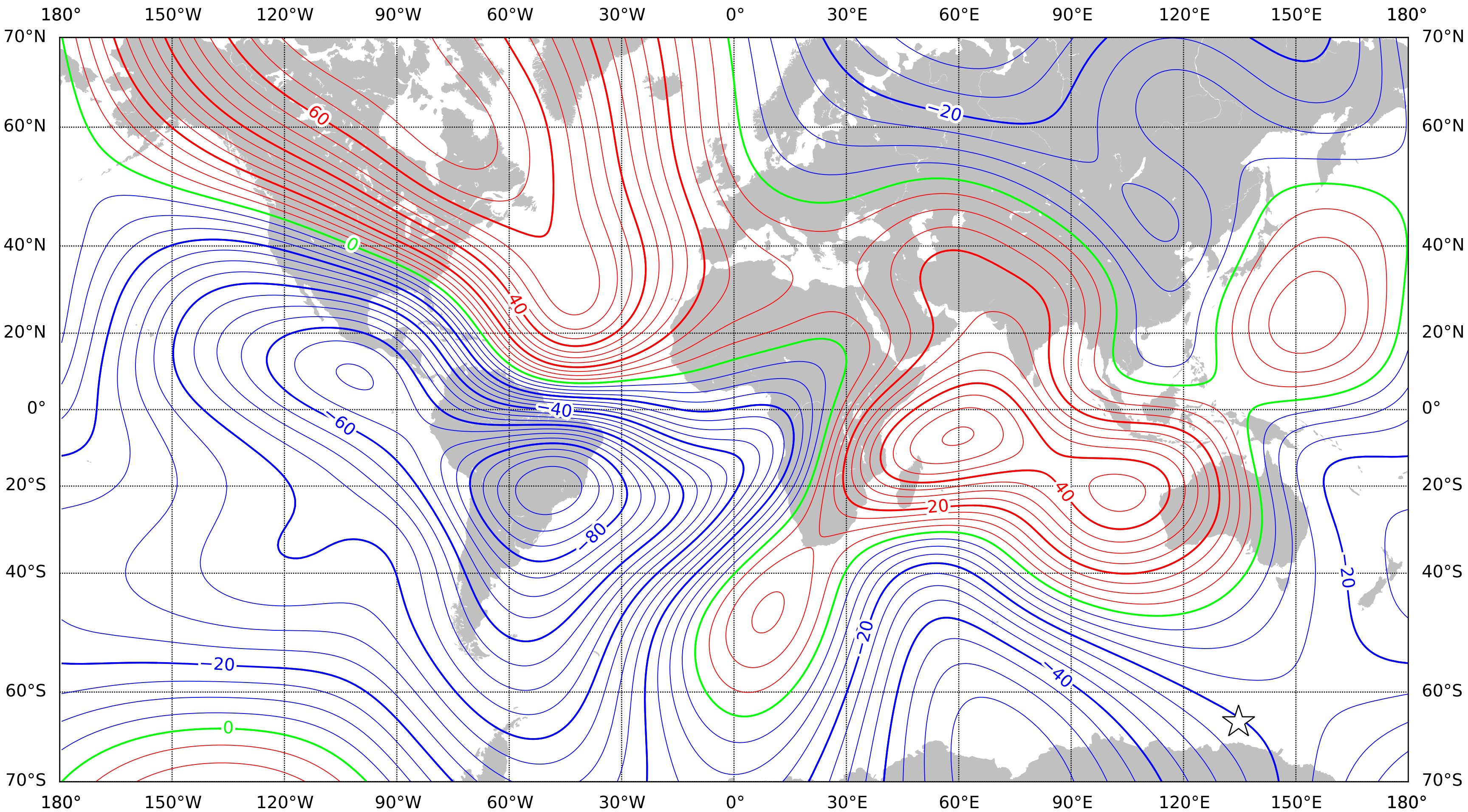
Annual rate of change of north component at 2027.5 from the World Magnetic Model - High Resolution (WMMHR) 2025 (core component only). Red - positive (northerly) change, blue - negative (southerly) change, green - zero change. Contour interval is 5nT/year, white star is the location of a magnetic pole and the projection is Mercator. This is an example of an isoporic chart. British Geological Survey © UKRI 2024
