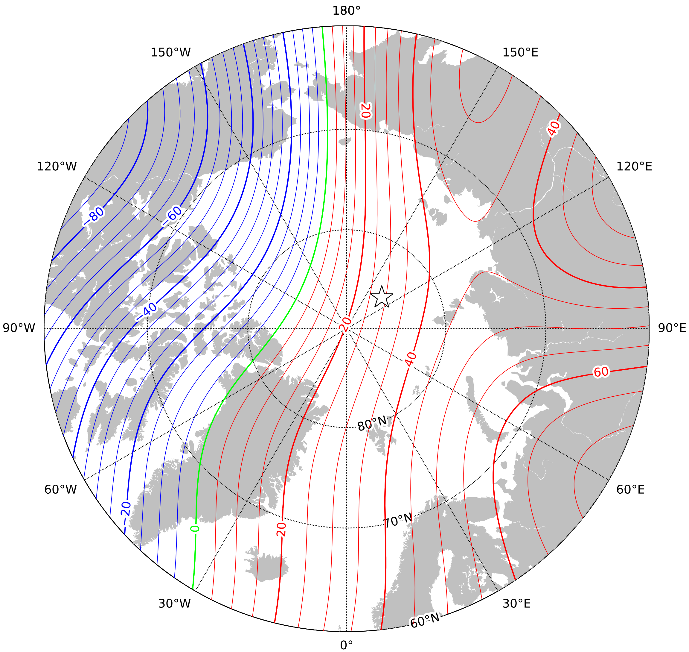
Annual rate of change of total intensity in the region of the north pole at 2027.5 from the World Magnetic Model - High Resolution (WMMHR) 2025 (core component only). Red - positive change, blue - negative change, green - zero change. Contour interval is 5nT/year, white star is the location of a magnetic pole and the projection is Polar Stereographic. This is an example of an isoporic chart. British Geological Survey © UKRI 2024
