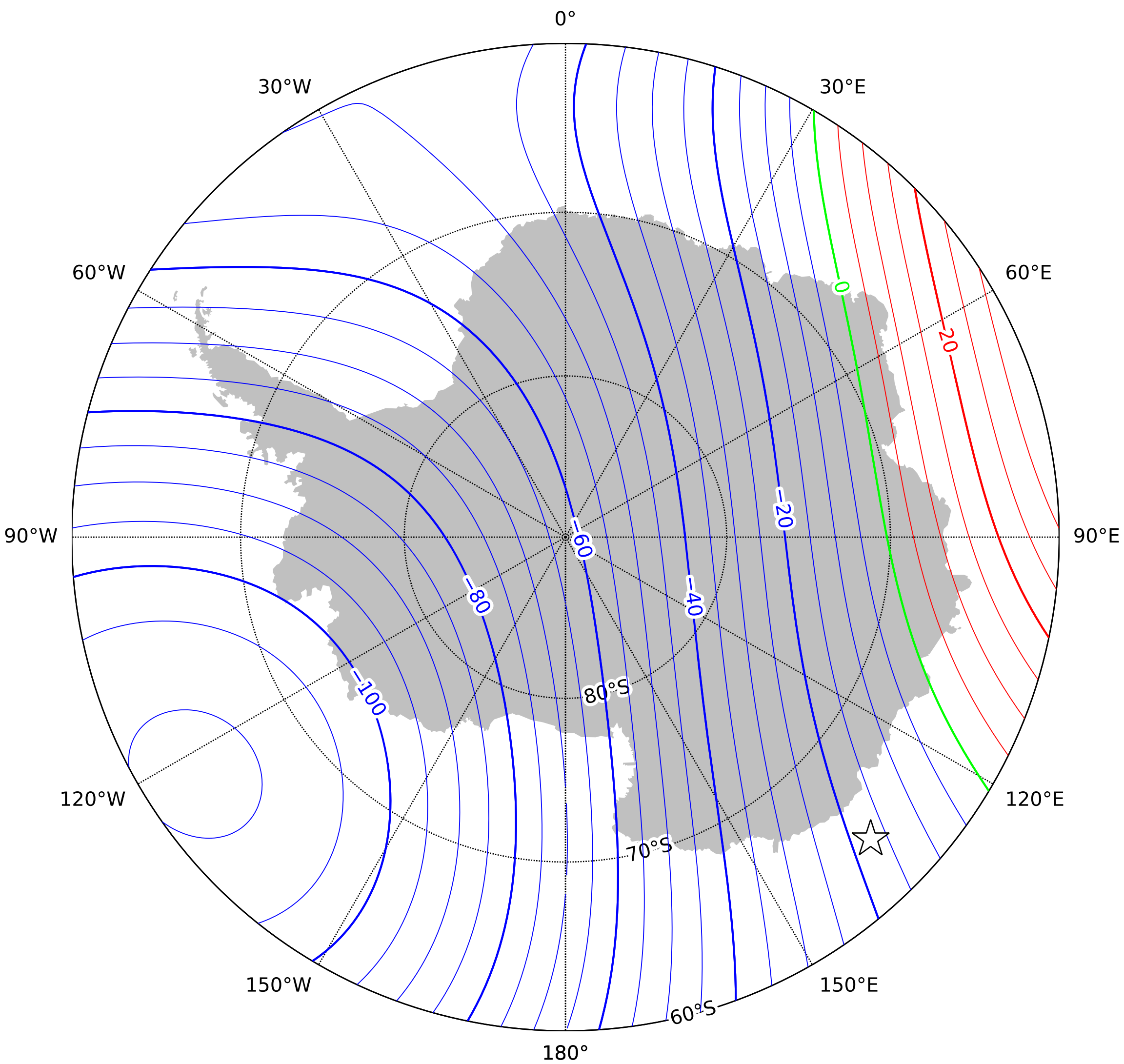
Annual rate of change of total intensity in the region of the south pole at 2027.5 from the World Magnetic Model - High Resolution (WMMHR) 2025 (core component only). Red - positive change, blue - negative change, green - zero change. Contour interval is 5nT/year, white star is the location of a magnetic pole and the projection is Polar Stereographic. This is an example of an isoporic chart. British Geological Survey © UKRI 2024
