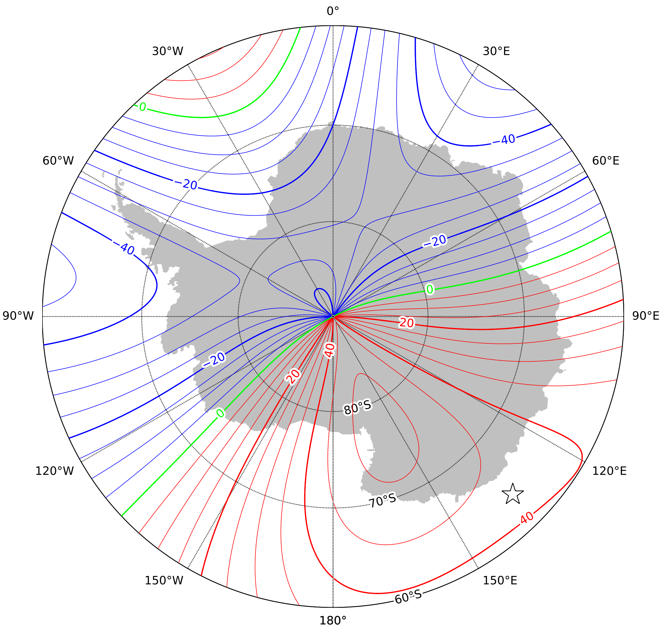
Annual rate of change of east component in the region of the south pole at 2027.5 from the World Magnetic Model - High Resolution (WMMHR) 2025 (core component only). Red - positive (easterly) change, blue - negative (westerly) change, green - zero change. Contour interval is 5nT/year, white star is the location of a magnetic pole and the projection is Polar Stereographic. This is an example of an isoporic chart. British Geological Survey © UKRI 2024
