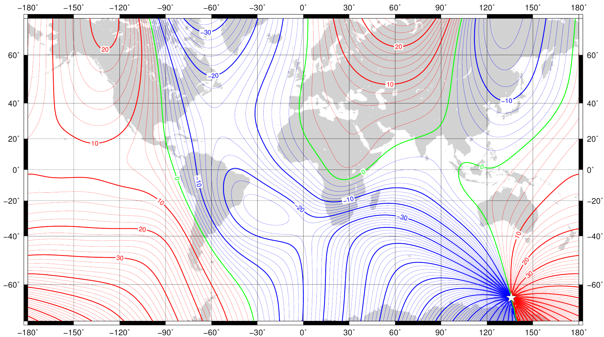
Declination (magnetic variation) at 2020.0 from the World Magnetic Model (WMM2020). Red – positive (east), blue – negative (west), green – zero (agonic line). Contour interval is 2°, white star is location of a magnetic pole and projection is Mercator. This is an example of an isogonic chart. Credit: British Geological Survey (UK Research and Innovation).
