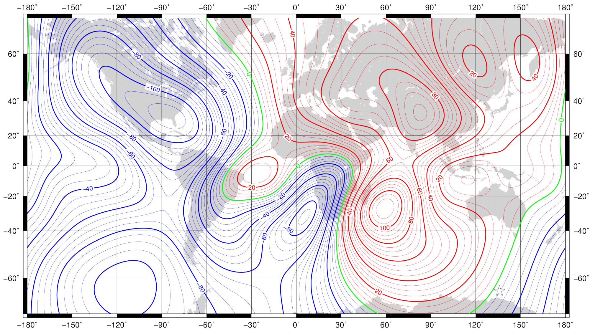
Annual rate of change of total intensity for 2020.0 to 2025.0 from the World Magnetic Model (WMM2020). Red – positive change, blue – negative change, green – zero change. Contour interval is 5 nT/year, white star is location of a magnetic pole and projection is Mercator. This is an example of an isoporic chart. Credit: British Geological Survey (UK Research and Innovation).
