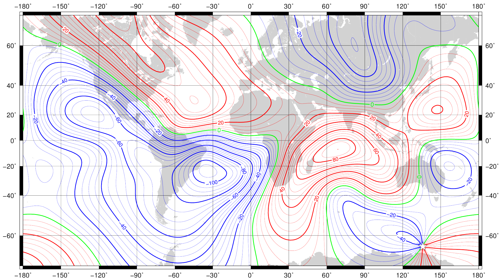
Annual rate of change of horizontal intensity for 2020.0 to 2025.0 from the World Magnetic Model (WMM2020). Red – positive change, blue – negative change, green – zero change. Contour interval is 5 nT/year, white star is location of a magnetic pole and projection is Mercator. This is an example of an isoporic chart. Credit: British Geological Survey (UK Research and Innovation).
