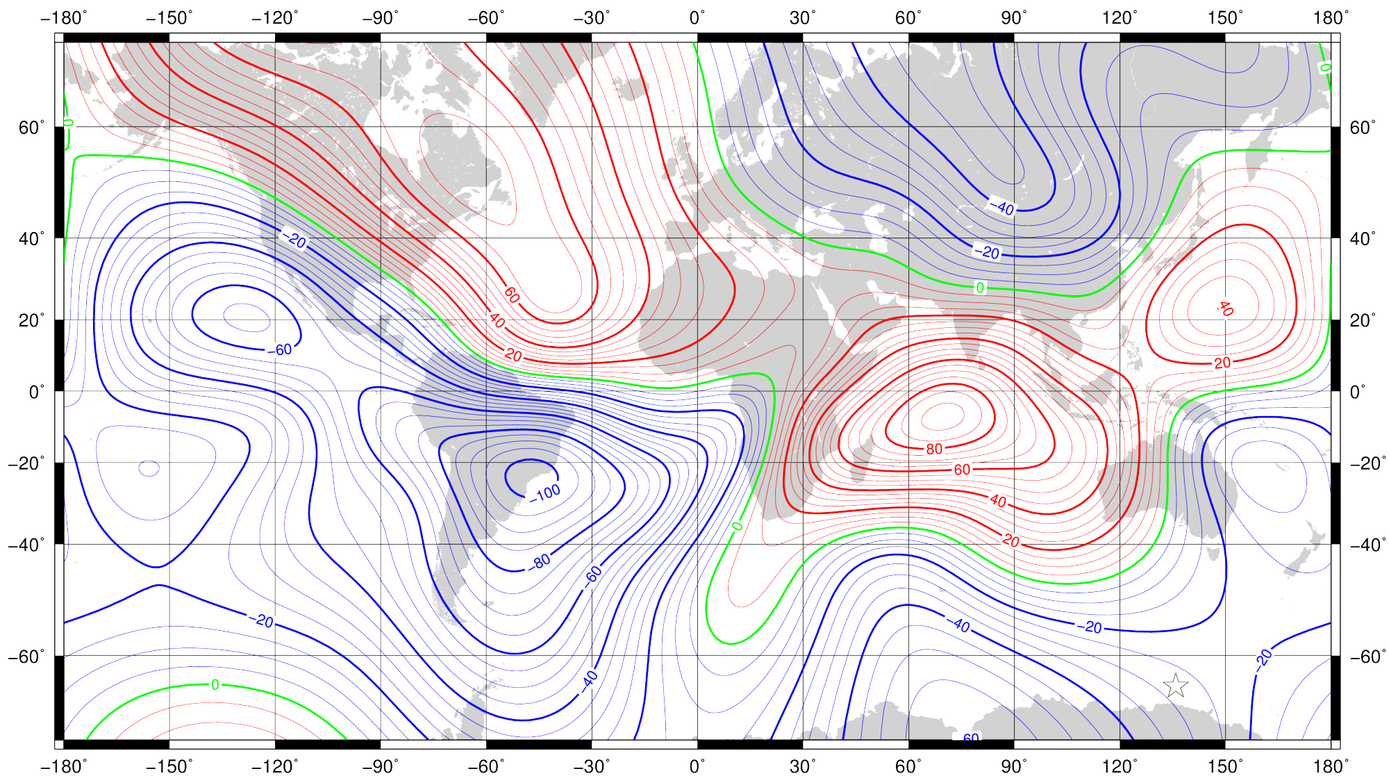
Annual rate of change of north component for 2020.0 to 2025.0 from the World Magnetic Model (WMM2020). Red – positive change, blue – negative change, green – zero change. Contour interval is 5 nT/year, white star is location of a magnetic pole and projection is Mercator. This is an example of an isoporic chart. Credit: British Geological Survey (UK Research and Innovation).
