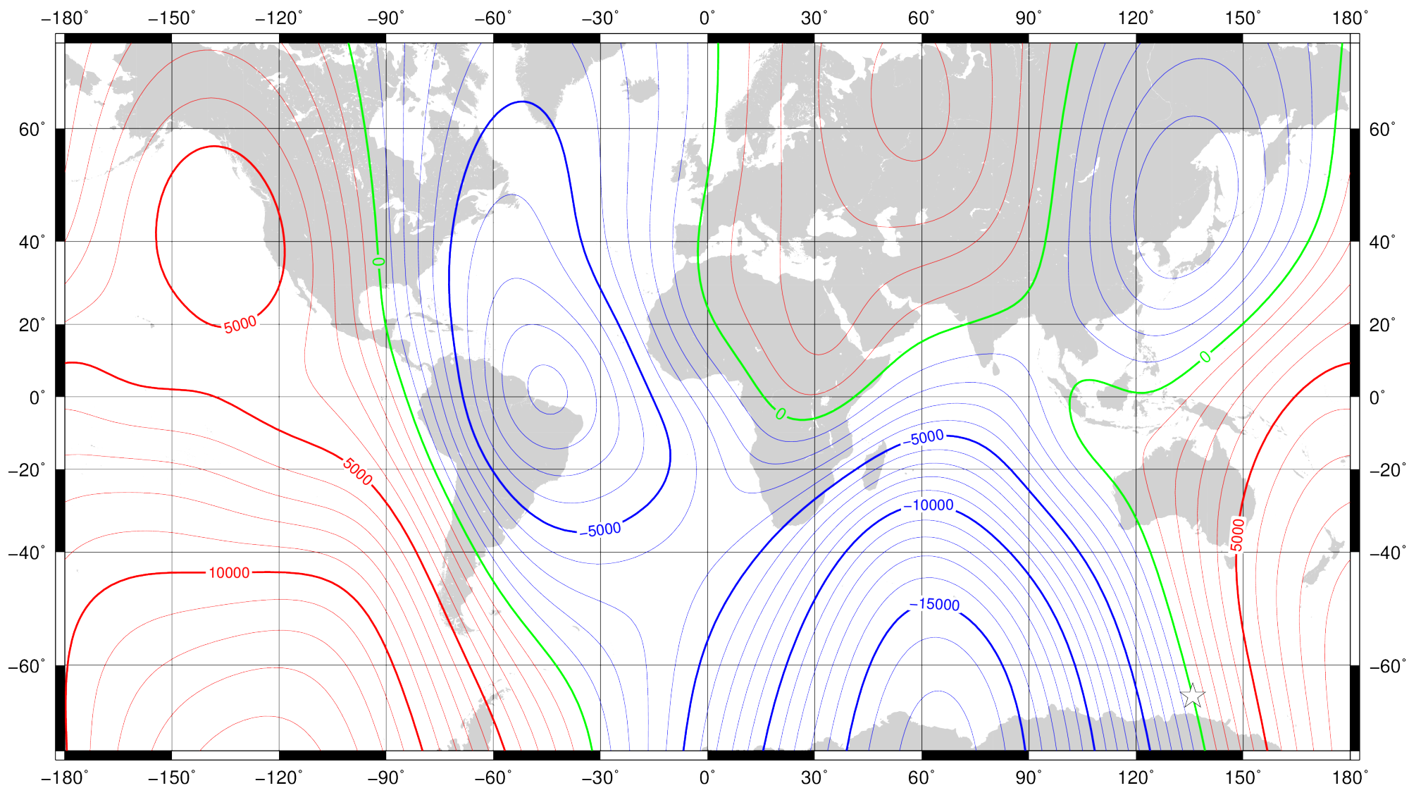
East component (Y) at 2020.0 from the World Magnetic Model (WMM2020). Red – positive (east), blue – negative (west), green – zero. Contour interval is 1000 nT, white star is location of a magnetic pole and projection is Mercator. This is an example of an isodynamic chart. Credit: British Geological Survey (UK Research and Innovation).
