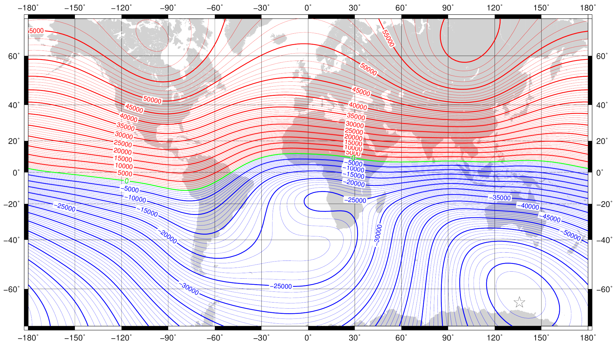
Vertical intensity ( Z ) at 2020.0 from the World Magnetic Model (WMM2020). Red – positive (down), blue – negative (up), green – zero. Contour interval is 1000 nT, white star is location of a magnetic pole and projection is Mercator. This is an example of an isodynamic chart. Credit: British Geological Survey (UK Research and Innovation).
