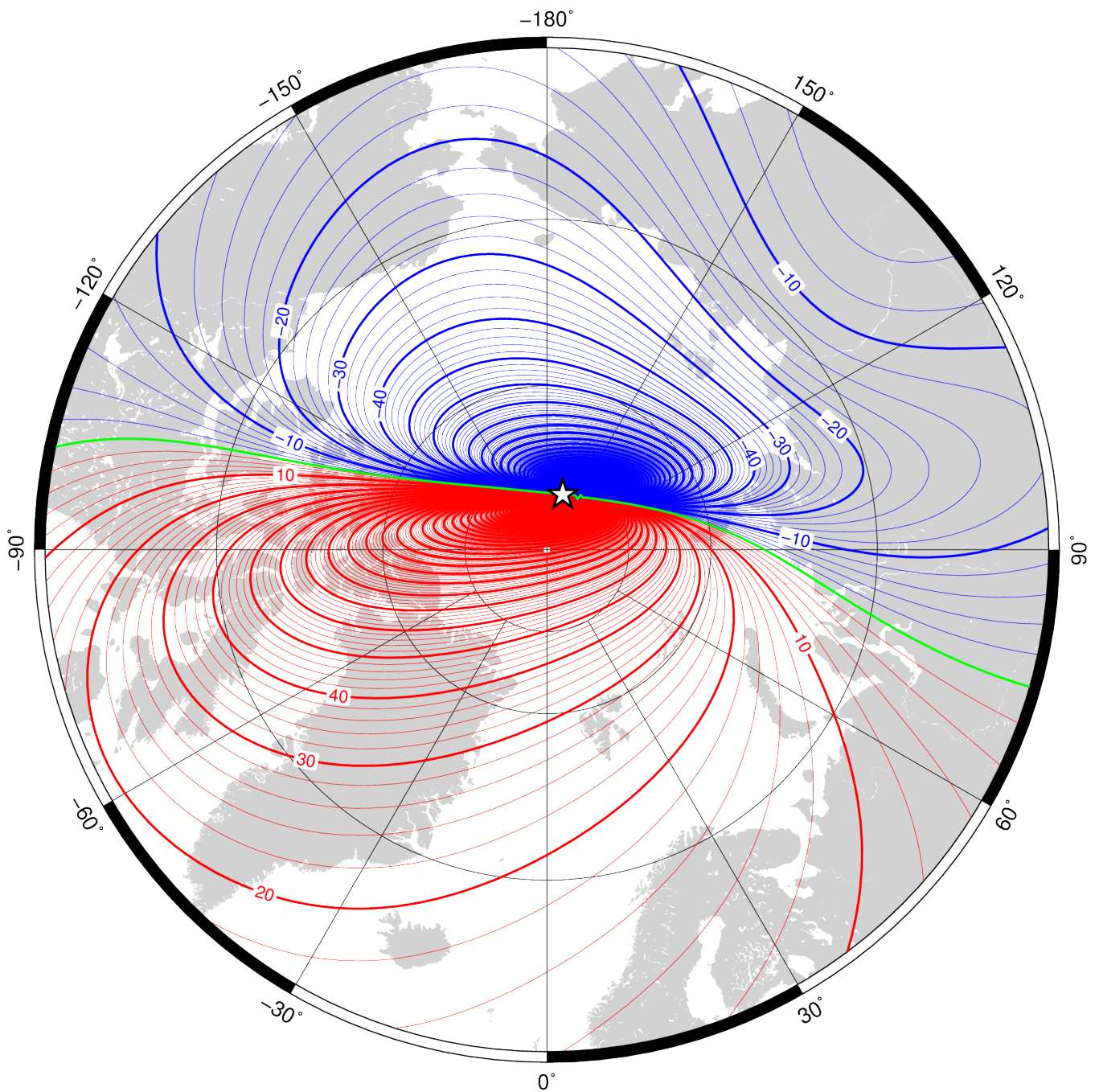
Annual rate of change of declination in region of north pole for 2020.0 to 2025.0 from the World Magnetic Model (WMM2020). Red – easterly change, blue – westerly change, green – zero change. Contour interval is 2'/year, white star is location of a magnetic pole and projection is Polar Stereographic. Credit: British Geological Survey (UK Research and Innovation).
