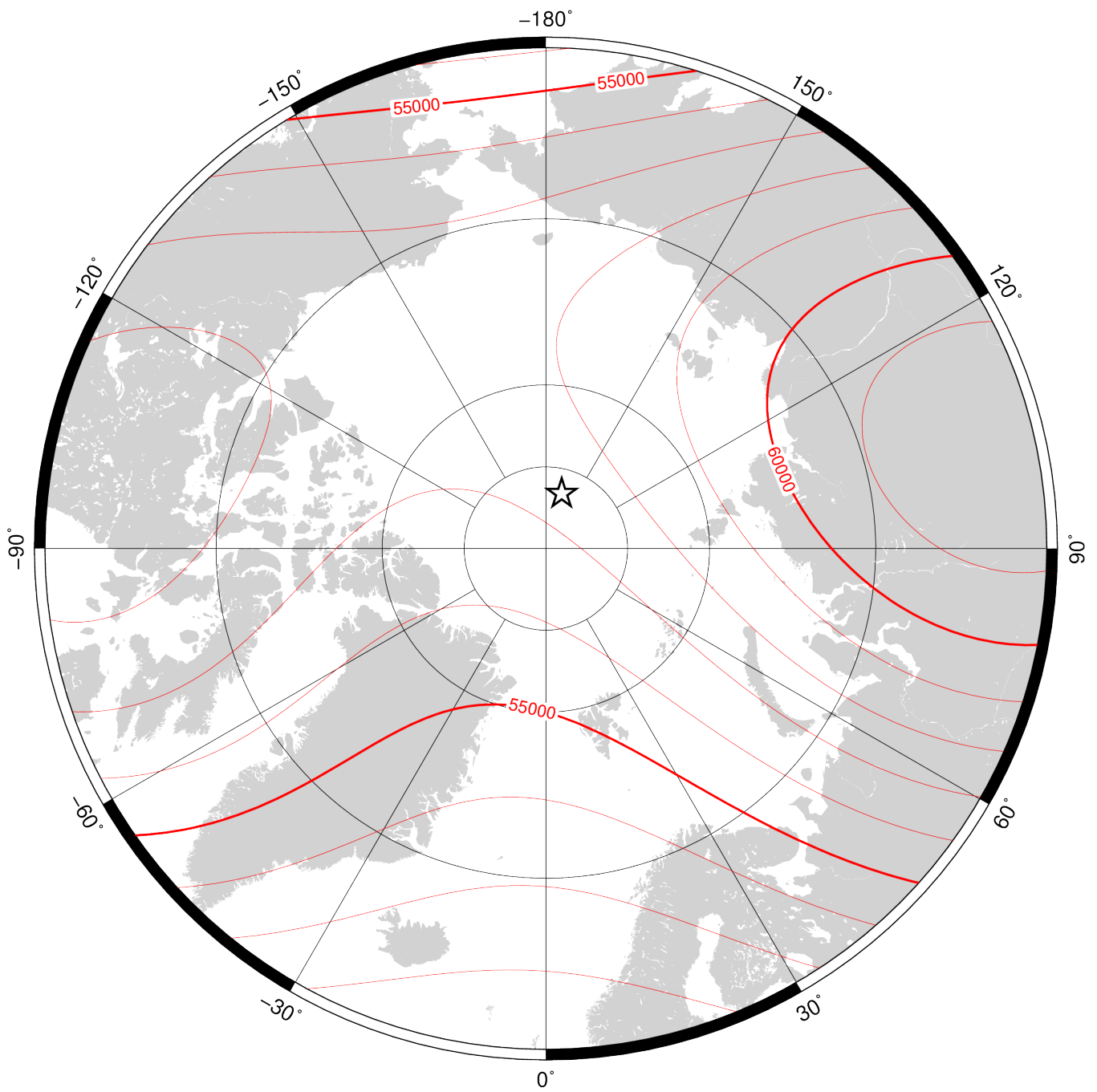
Total intensity ( F ) in region of north pole at 2020.0 from the World Magnetic Model (WMM2020). Contour interval is 1000 nT, white star is location of a magnetic pole and projection is Polar Stereographic. Credit: British Geological Survey (UK Research and Innovation).
