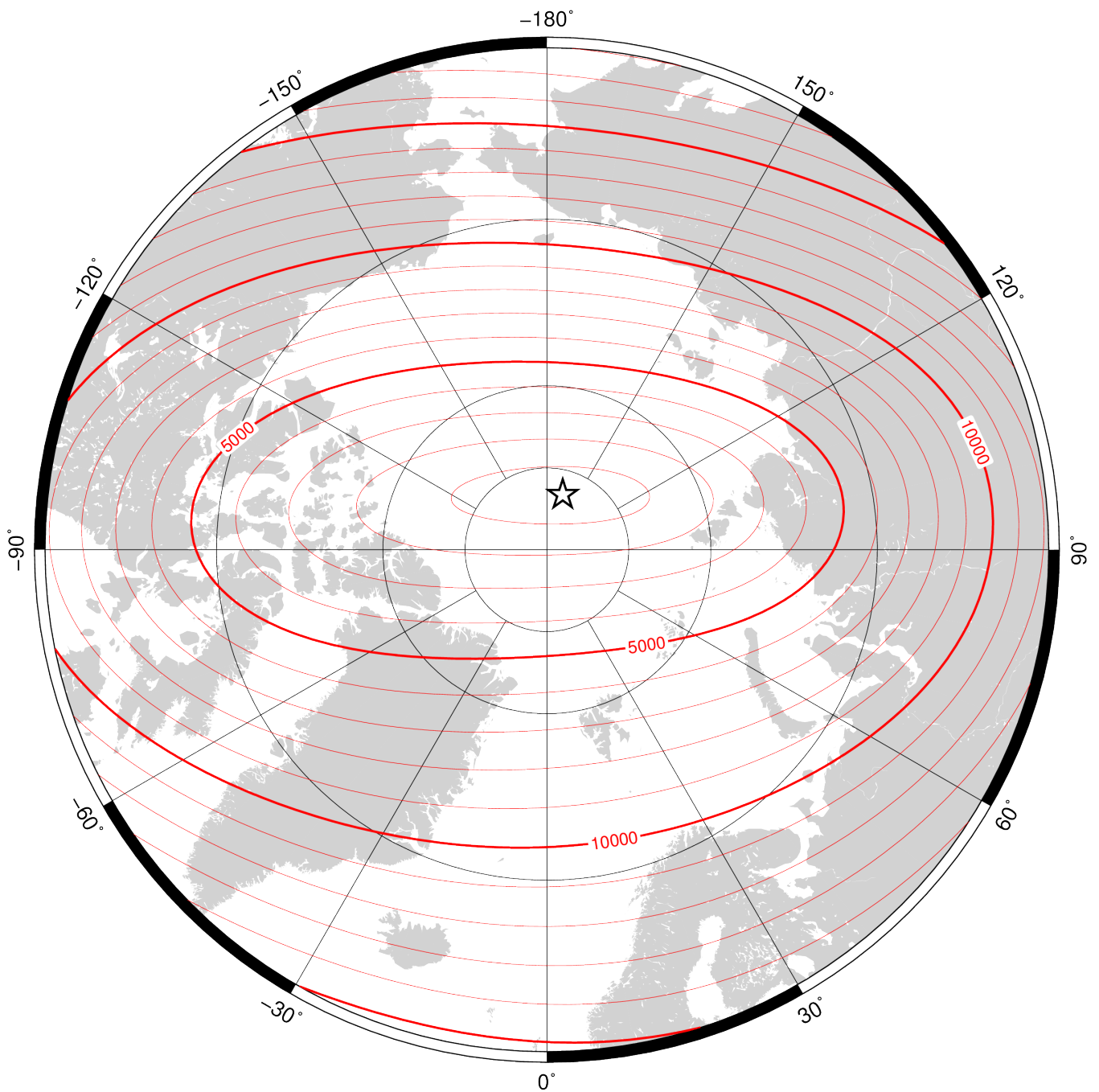
Horizontal intensity ( H ) in region of north pole at 2020.0 from the World Magnetic Model (WMM2020). Contour interval is 1000 nT, white star is location of a magnetic pole and projection is Polar Stereographic. Credit: British Geological Survey (UK Research and Innovation).
