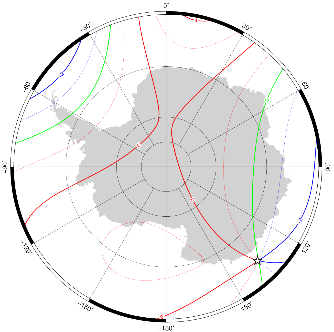
Annual rate of change of inclination in region of south pole for 2020.0 to 2025.0 from the World Magnetic Model (WMM2020). Red – positive change, blue – negative change, green – zero change. Contour interval is 1'/year, white star is location of a magnetic pole and projection is Polar Stereographic. Credit: British Geological Survey (UK Research and Innovation).
