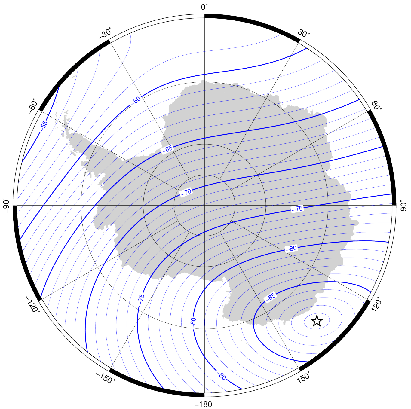
Inclination (magnetic dip) in region of south pole at 2020.0 from the World Magnetic Model (WMM2020). Contour interval is 1^\circ , white star is location of a magnetic pole and projection is Polar Stereographic. Credit: British Geological Survey (UK Research and Innovation).
